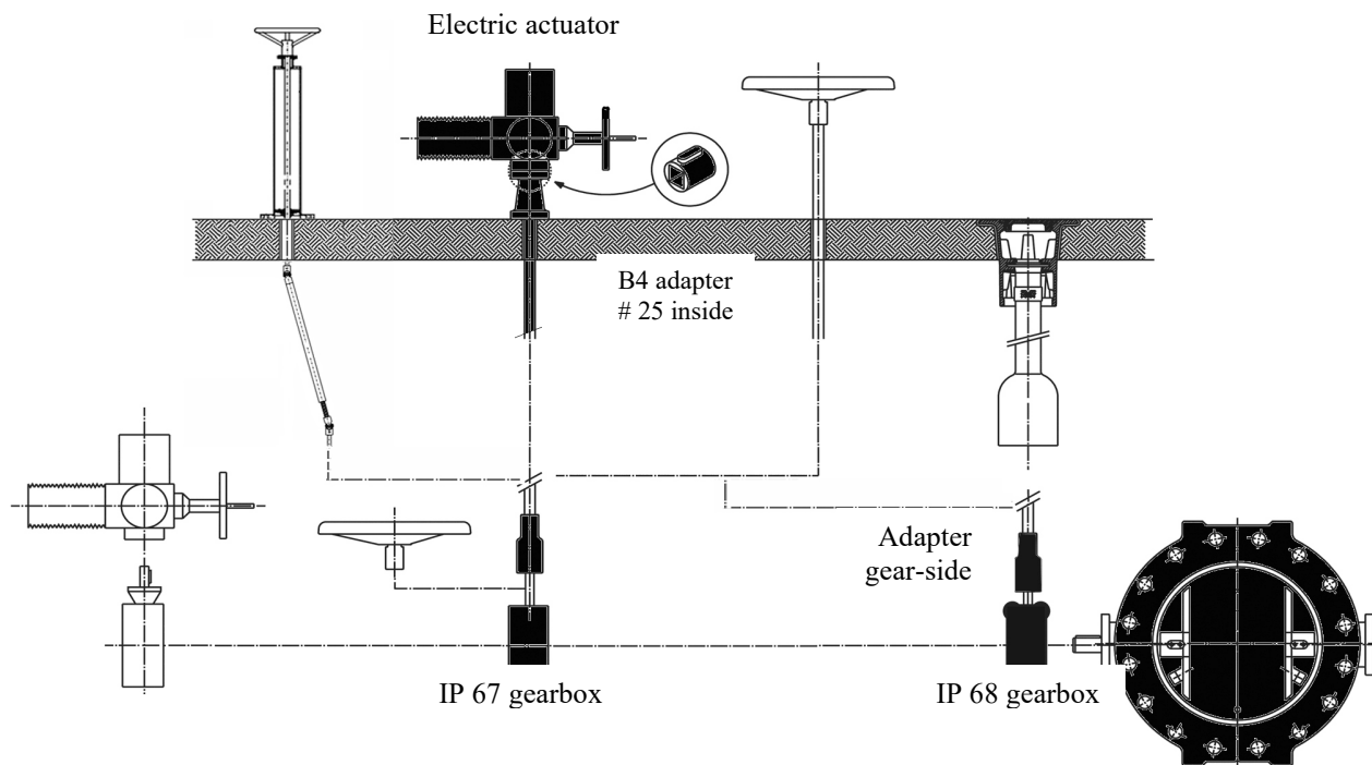
Butterfly valve DN 200-1200
